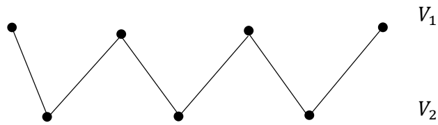
Figure 1.5.6 A diagram of a bipartite graph
