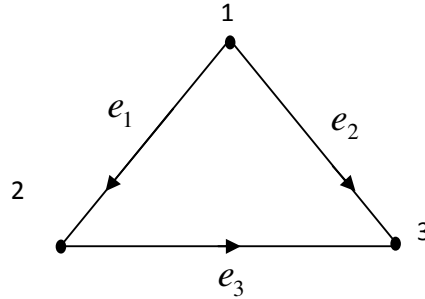
Figure 1.5.2 A diagram of the simple graph G .
