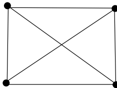
Figure 1.5.5 A diagram of the complete graph K_4
