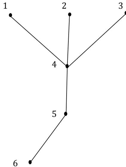
Figure 1.5.11 a diagram of tree
